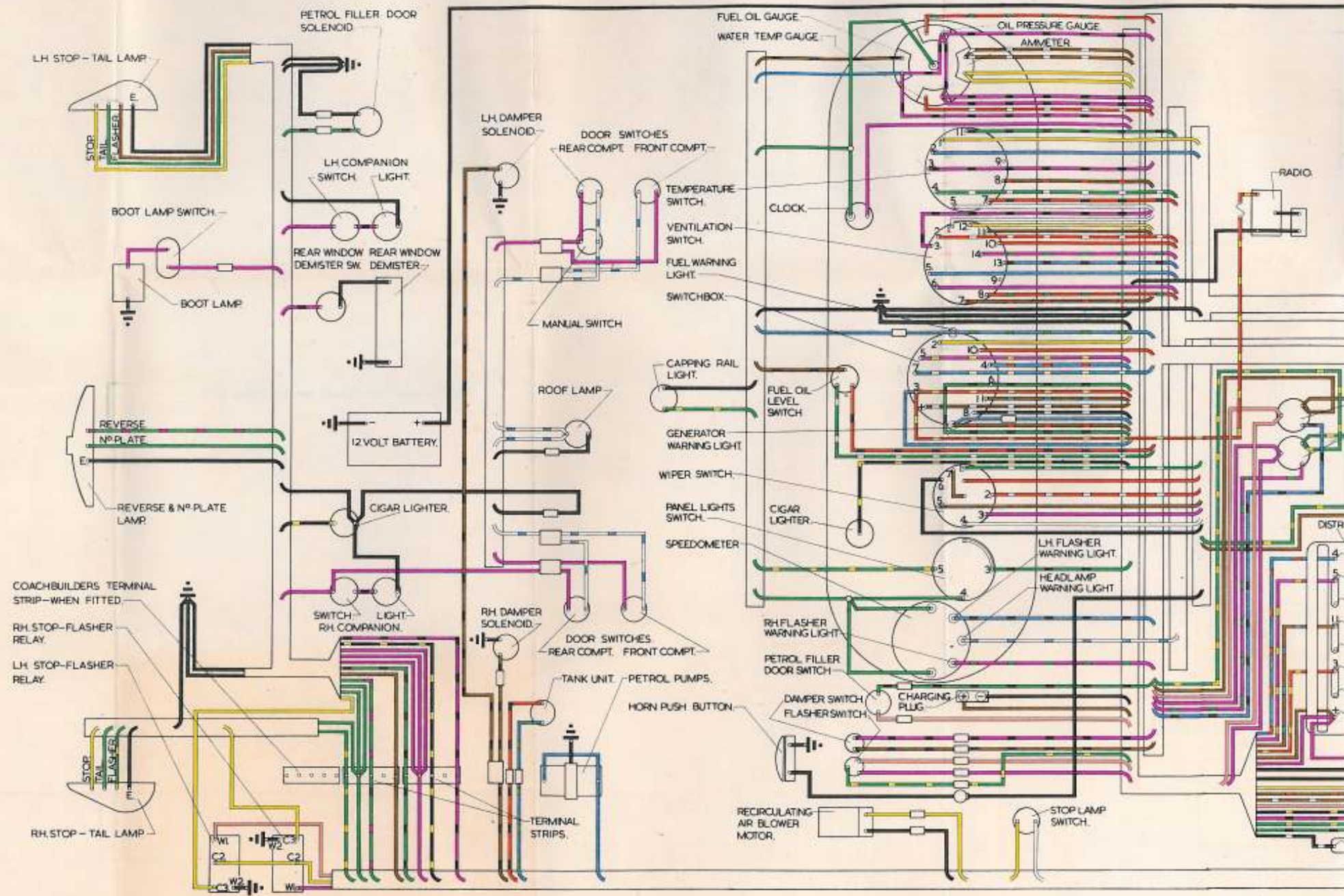
WIRING DIAGRAM
