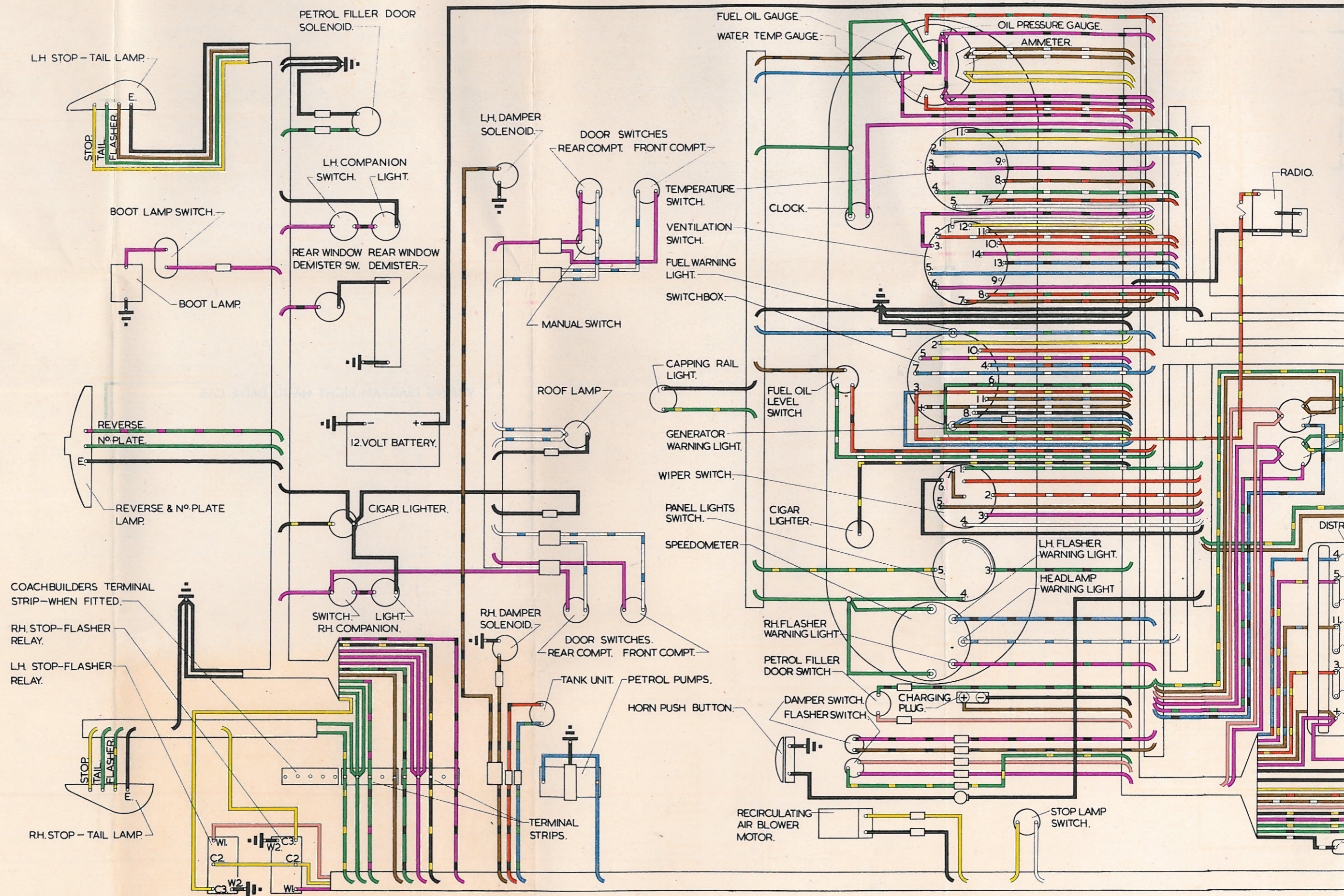
WIRING DIAGRAM
