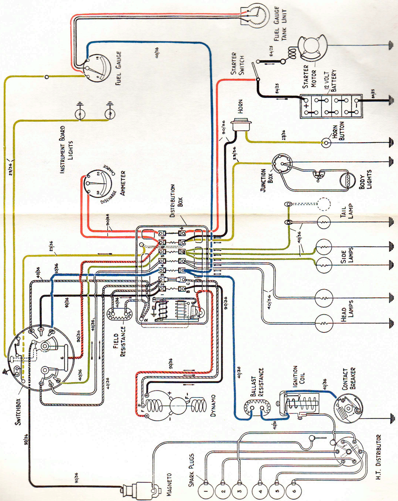
Fig 34.—ELECTRICAL WIRING DIAGRAM. (CHASSIS NOS. GBT, GKT, GAU, GMU, GZU, GHW, GRW and GAW.)
