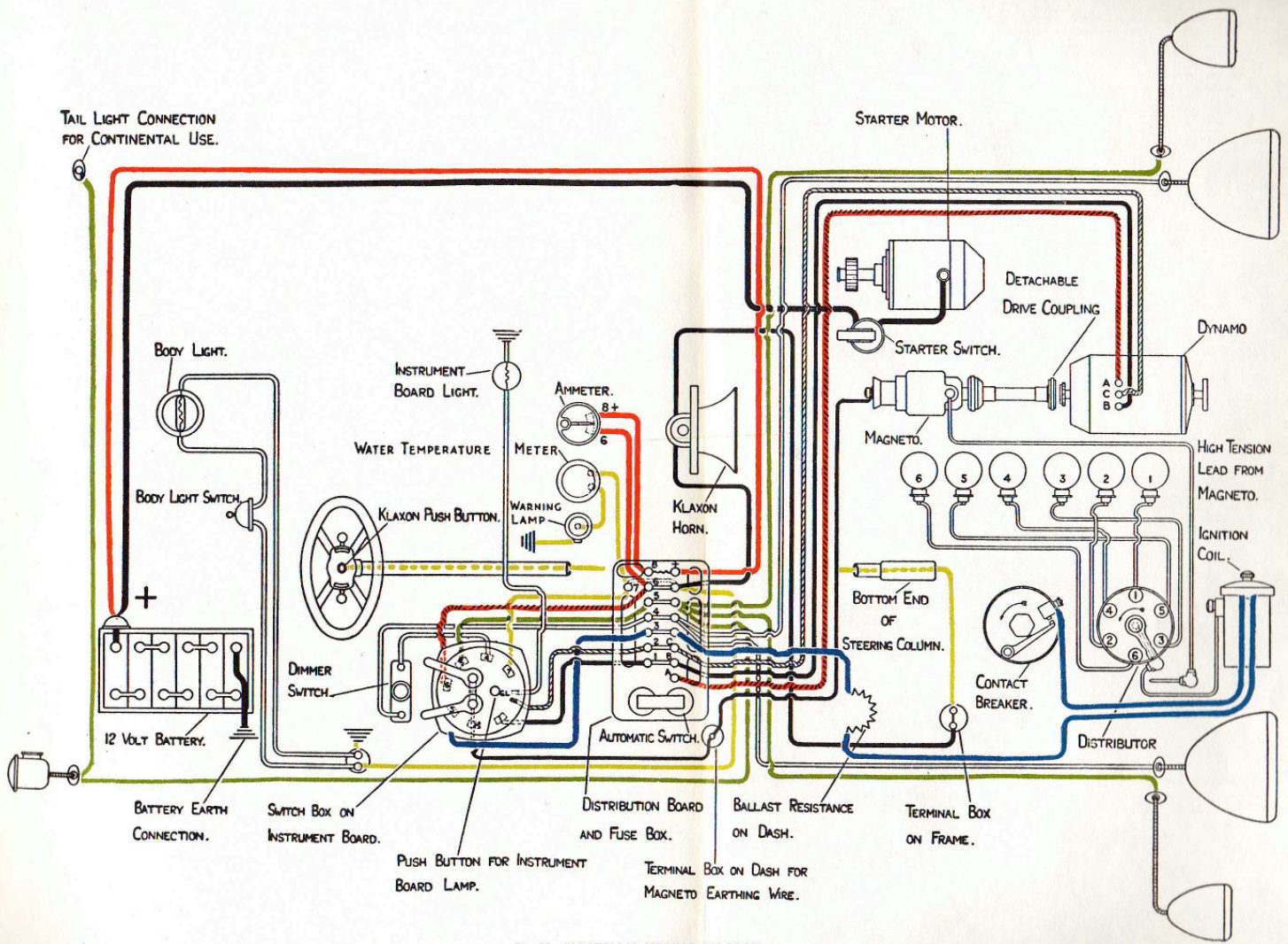
Fig. 33—ELECTRICAL WIRING DIAGRAM. CHASSIS NOS. GXO, GGP, GDP, GWP, GLR, GSR, GTR, GNS, GOS, GPS, GFT.)
