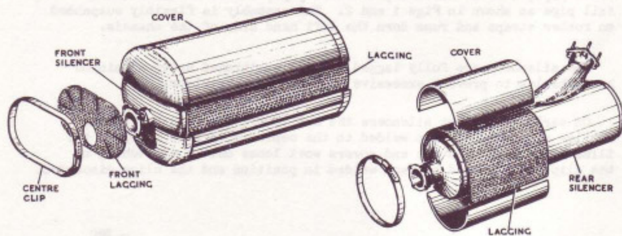
FIG. 2. FRONT AND REAR SILENCERS.
