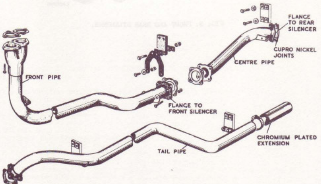
FIG. 1. EXHAUST PIPES
