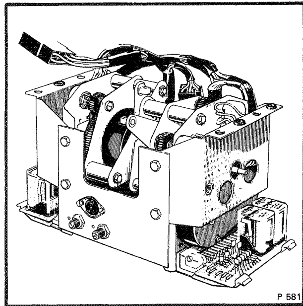
Servo assembly
